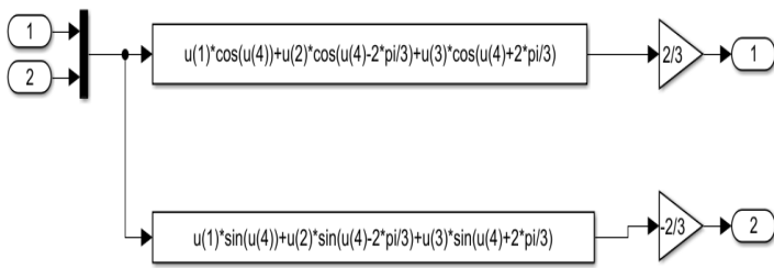
Figure 4. Simulation model of Park transform
