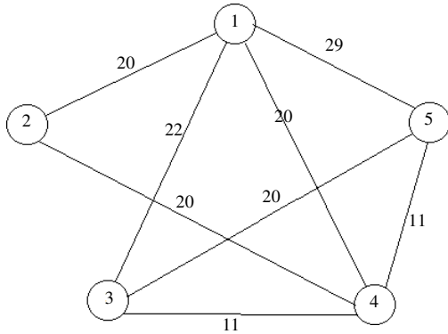
Fig. 1: Graph of affinity
