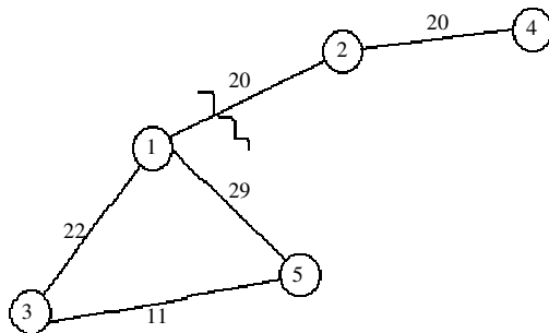
Fig. 2: Results fragmentation GBVP Algorithm, starting from node 1
