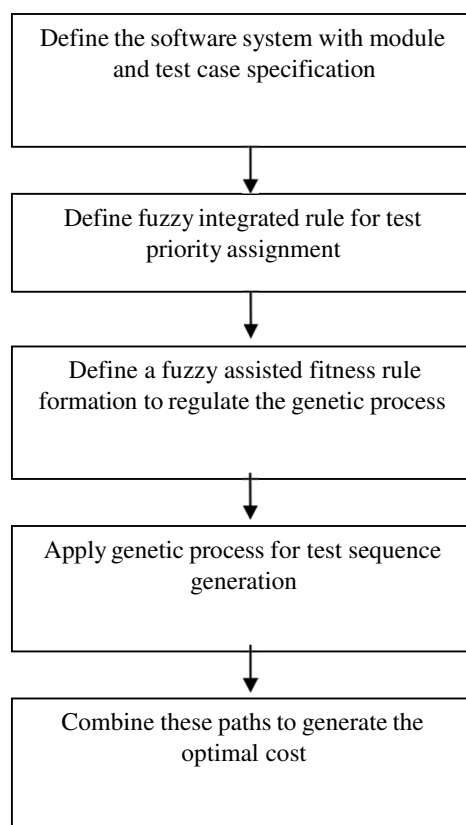
Figure 2: Proposed Model
